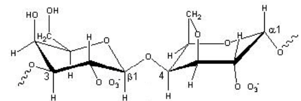
B-Galactopyranose and \alpha -Galactopyranose units
